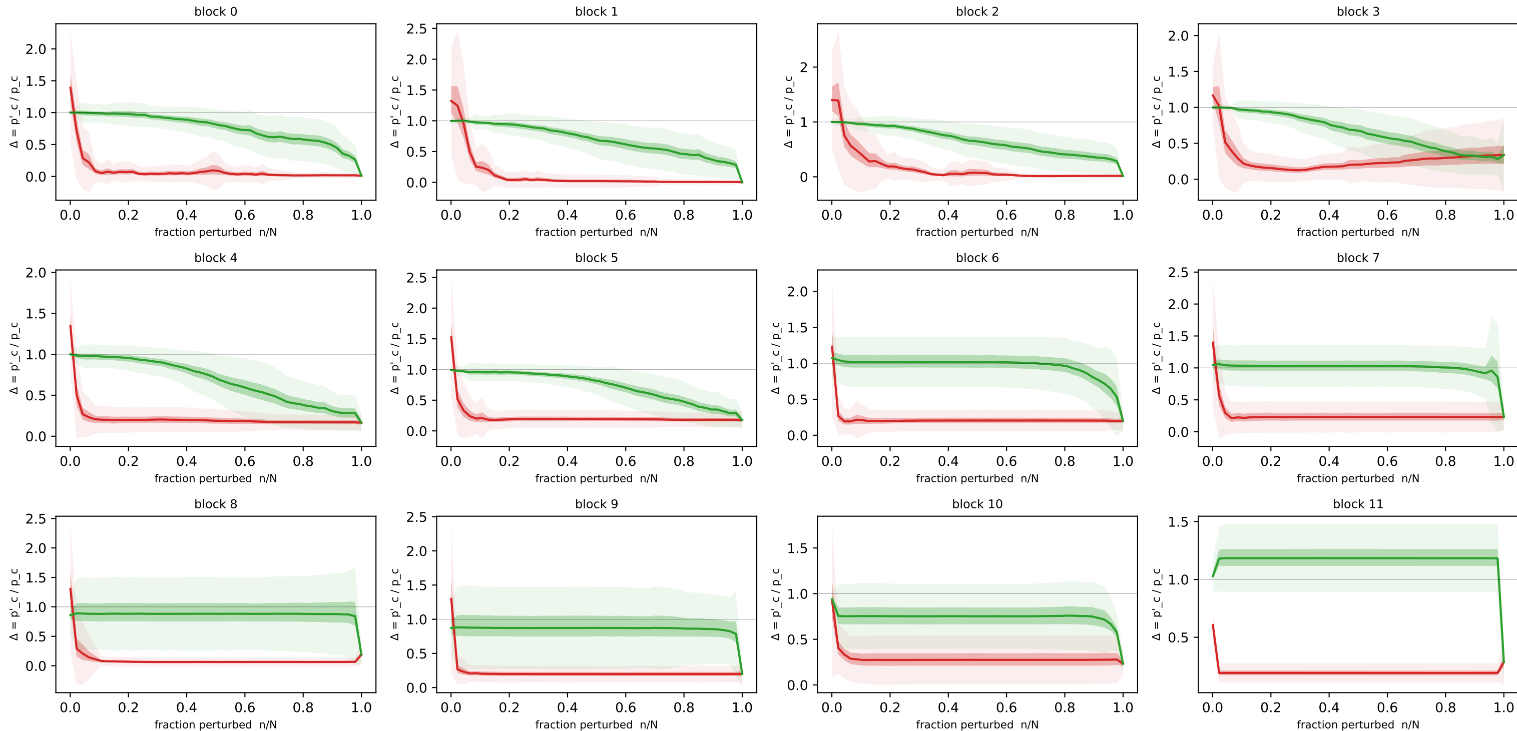
Concept-flipping curves — funny_birds · residual · SAE m=1536 (n=60 imgs, N=1536 detectors)
