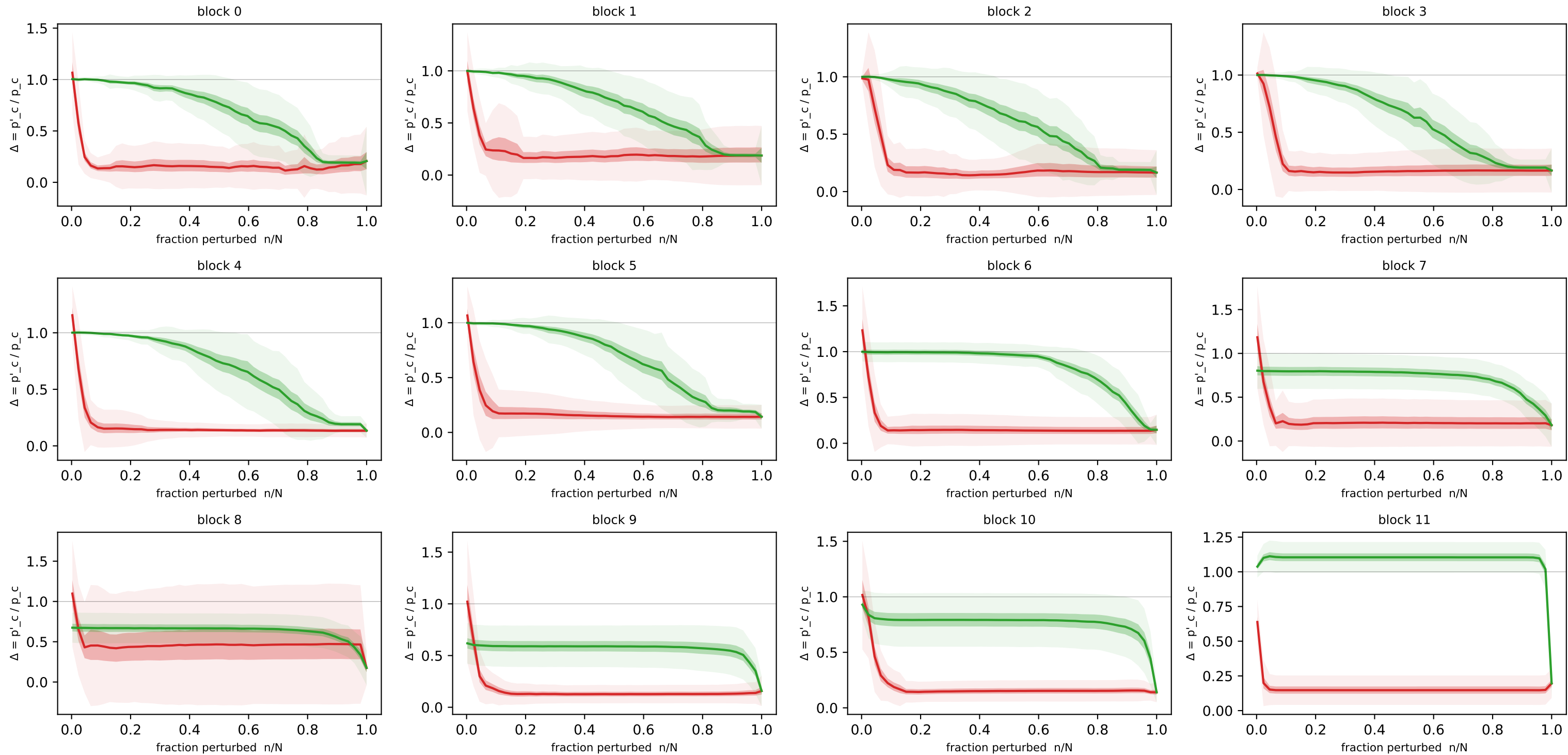
Concept-flipping curves — funny_birds · residual · SAE m=384 (n=60 imgs, N=384 detectors)
