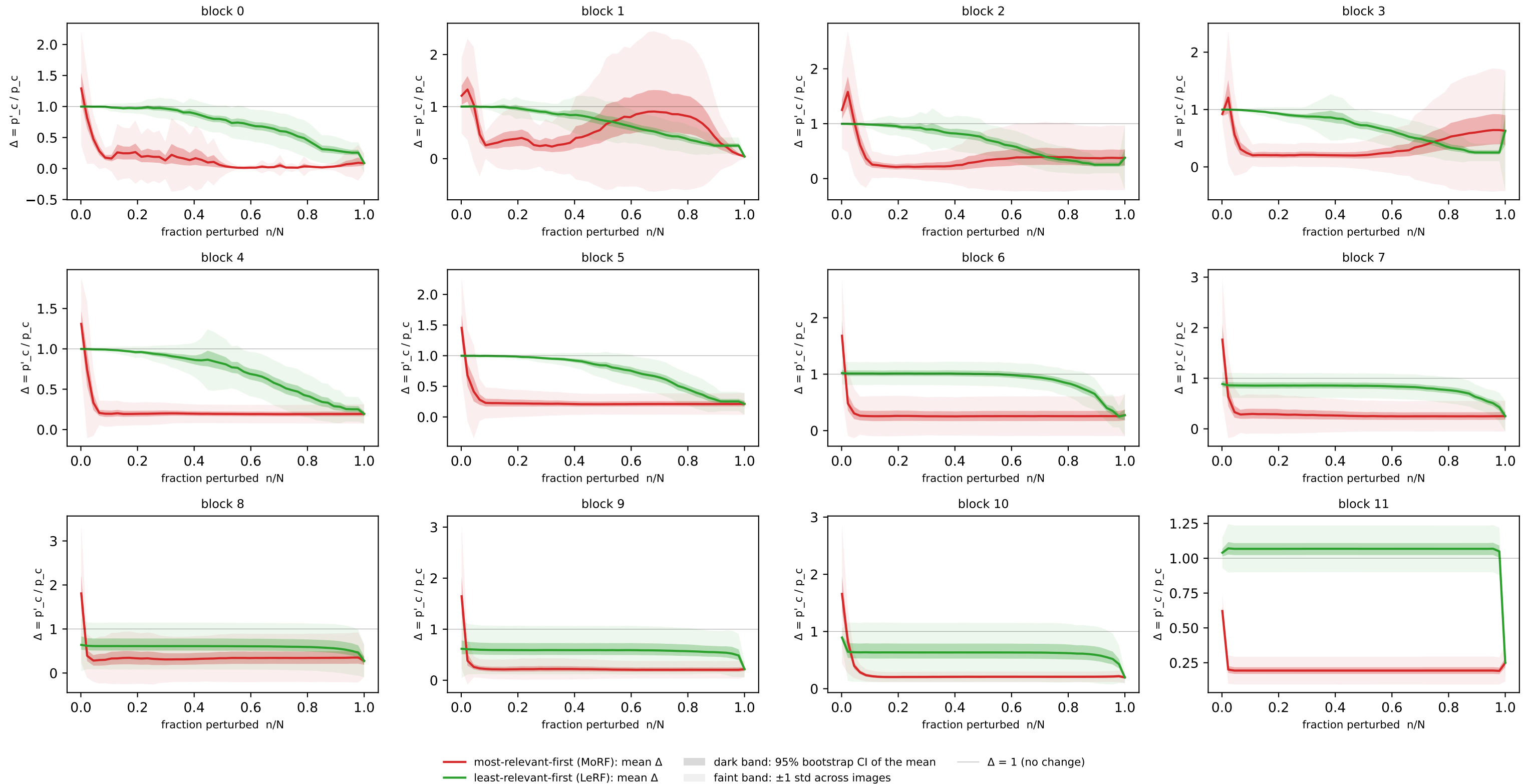
Concept-flipping curves — funny_birds · residual · SAE m=768 (n=60 imgs, N=768 detectors)
