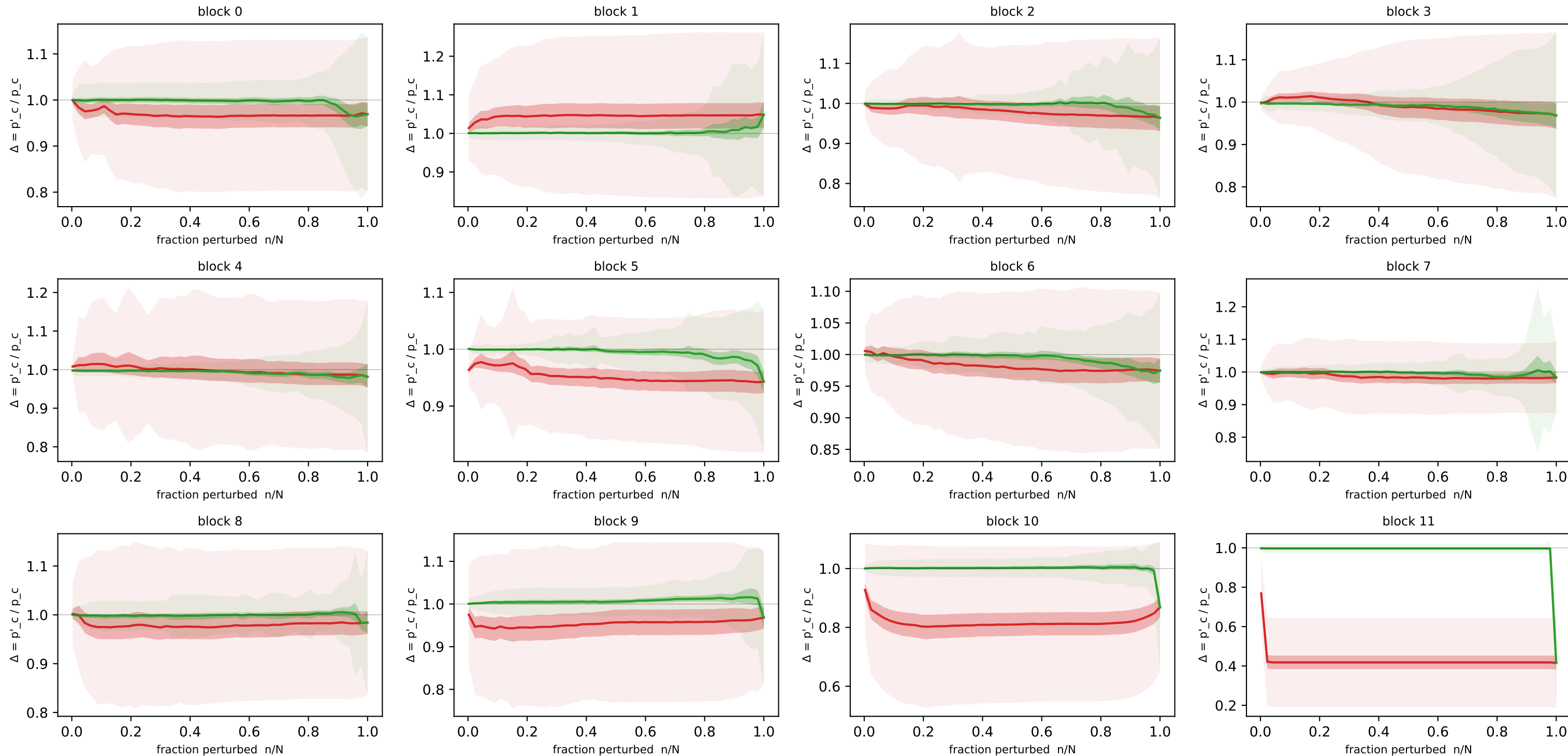
Concept-flipping curves — imagenet · proj_drop · SAE m=384 (n=158 imgs, N=384 detectors)
