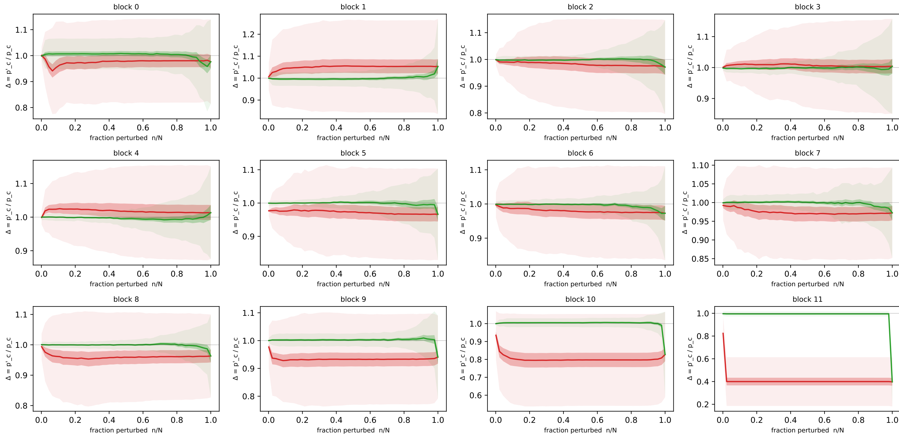
Concept-flipping curves — imagenet · proj_drop · SAE m=768 (n=158 imgs, N=768 detectors)
