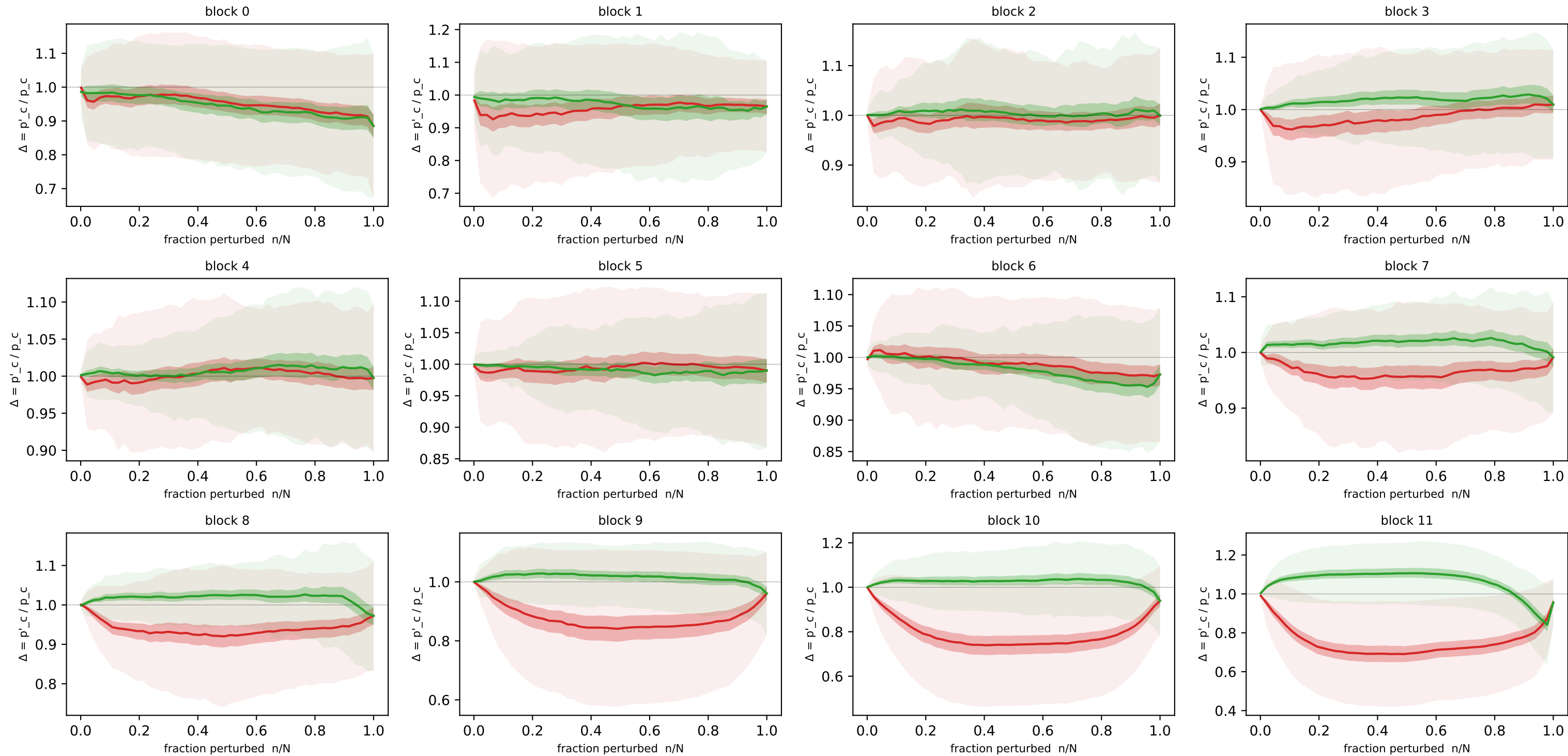
Concept-flipping curves — imagenet · proj_drop · no SAE (axis-aligned, 768) (n=158 imgs, N=768 detectors)
