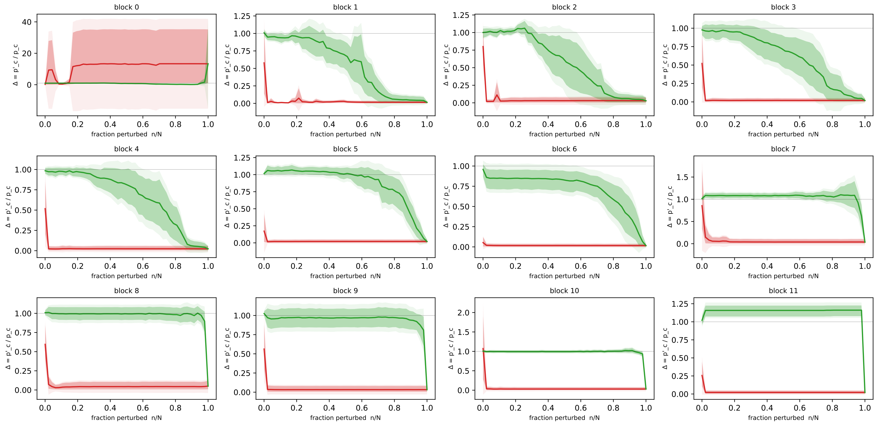
Concept-flipping curves — imagenet · residual · SAE m=3072 (n=8 imgs, N=3072 detectors)
