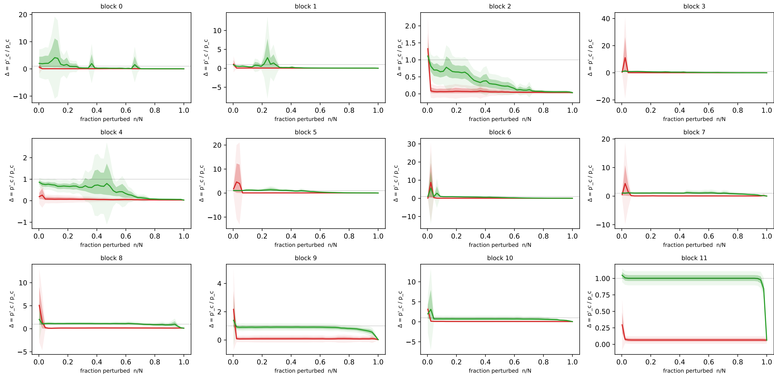
Concept-flipping curves — imagenet · residual · SAE m=384 (n=20 imgs, N=384 detectors)
