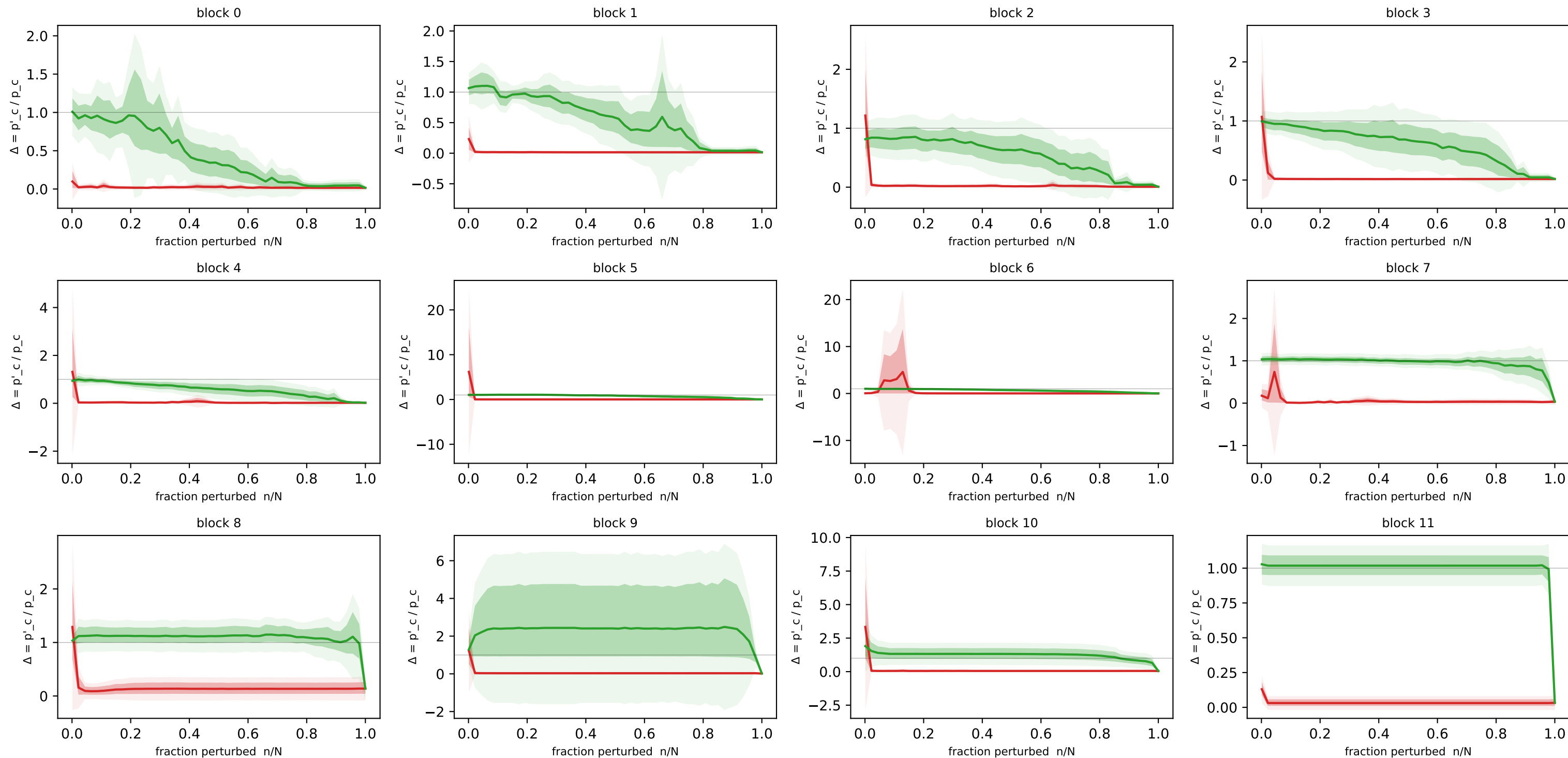
Concept-flipping curves — imagenet · residual · SAE m=768 (n=16 imgs, N=768 detectors)
