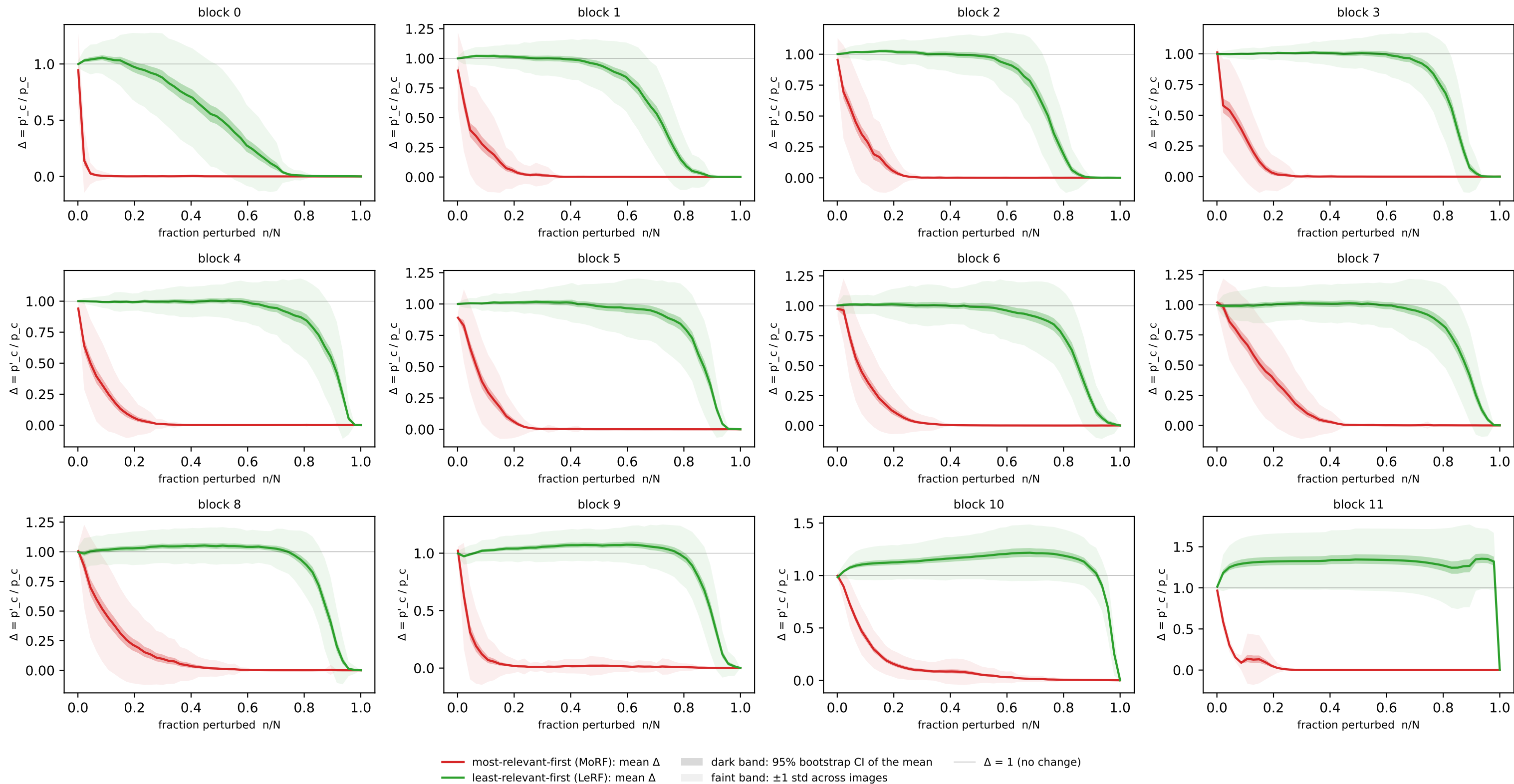
Concept-flipping curves — imagenet · residual · no SAE (axis-aligned, 768) (n=158 imgs, N=768 detectors)
