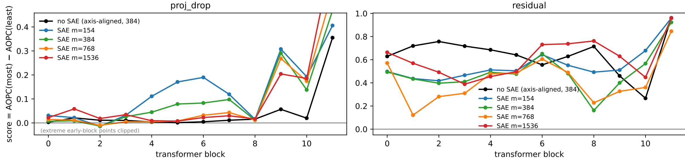
Concept-flipping score per block vs SAE dimensionality — funny_birds higher \Rightarrow MoRF collapses faster than LeRF (more faithful & concentrated relevance)
