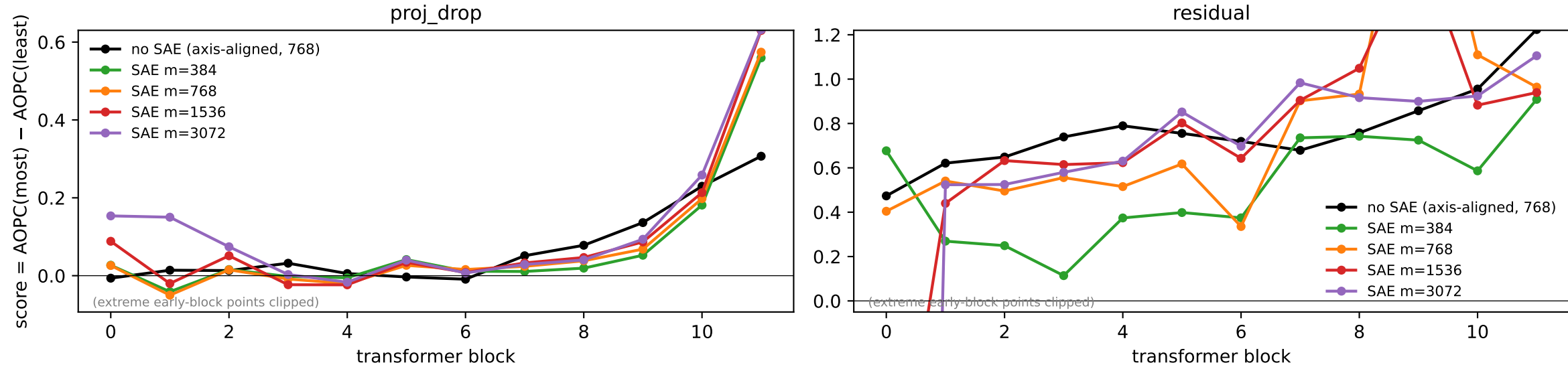
Concept-flipping score per block vs SAE dimensionality — imagenet higher \Rightarrow MoRF collapses faster than LeRF (more faithful & concentrated relevance)
