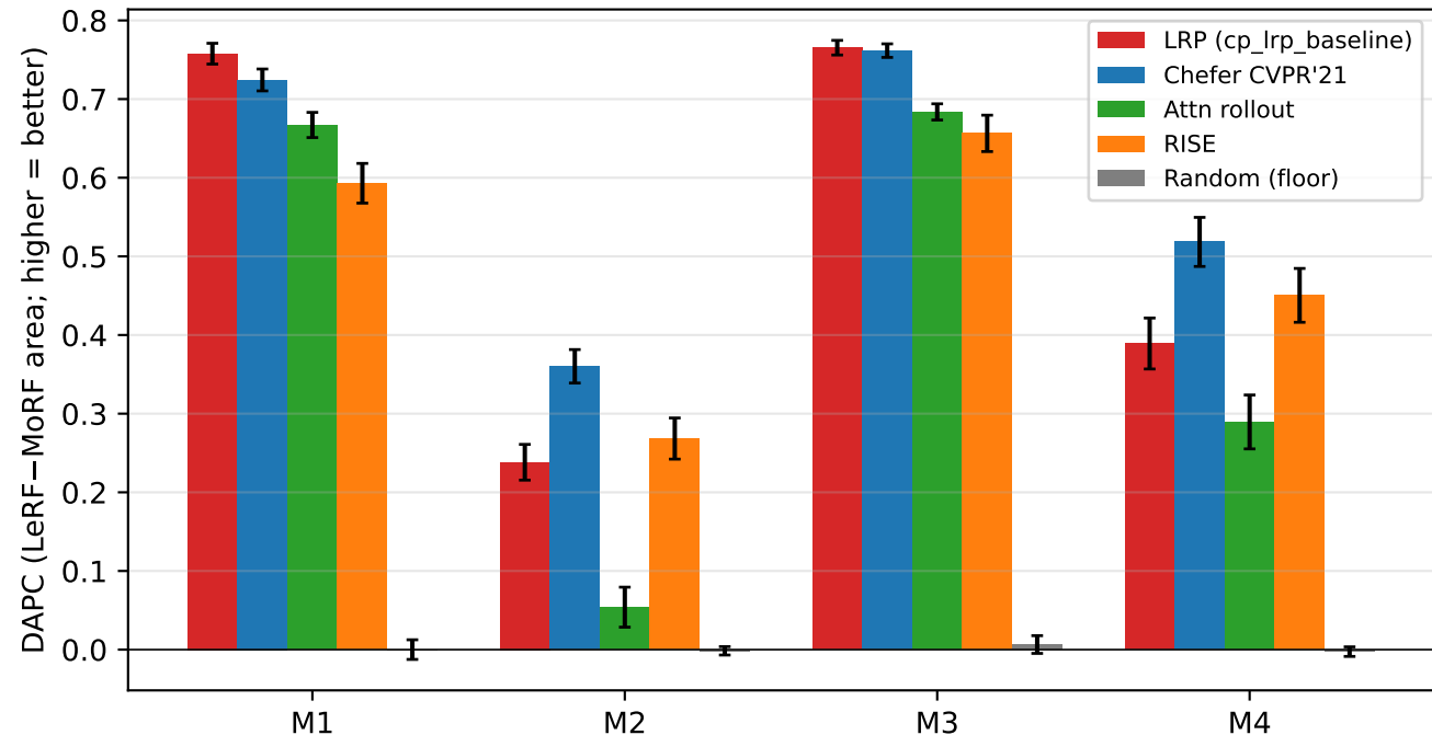
Insertion-Deletion DAPC per method × model
