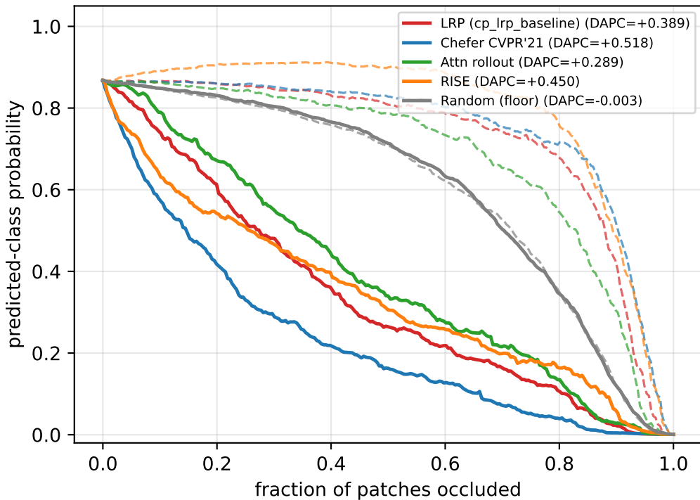
M4: DINOv3-B/16 (+reg, canvit head) · ImageNet (val) MoRF (solid) vs LeRF (dashed)
