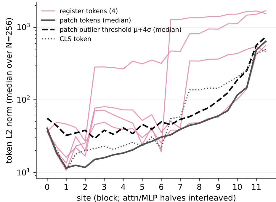
M3 DINOv3-S (+reg, finetuned) · FunnyBirds
