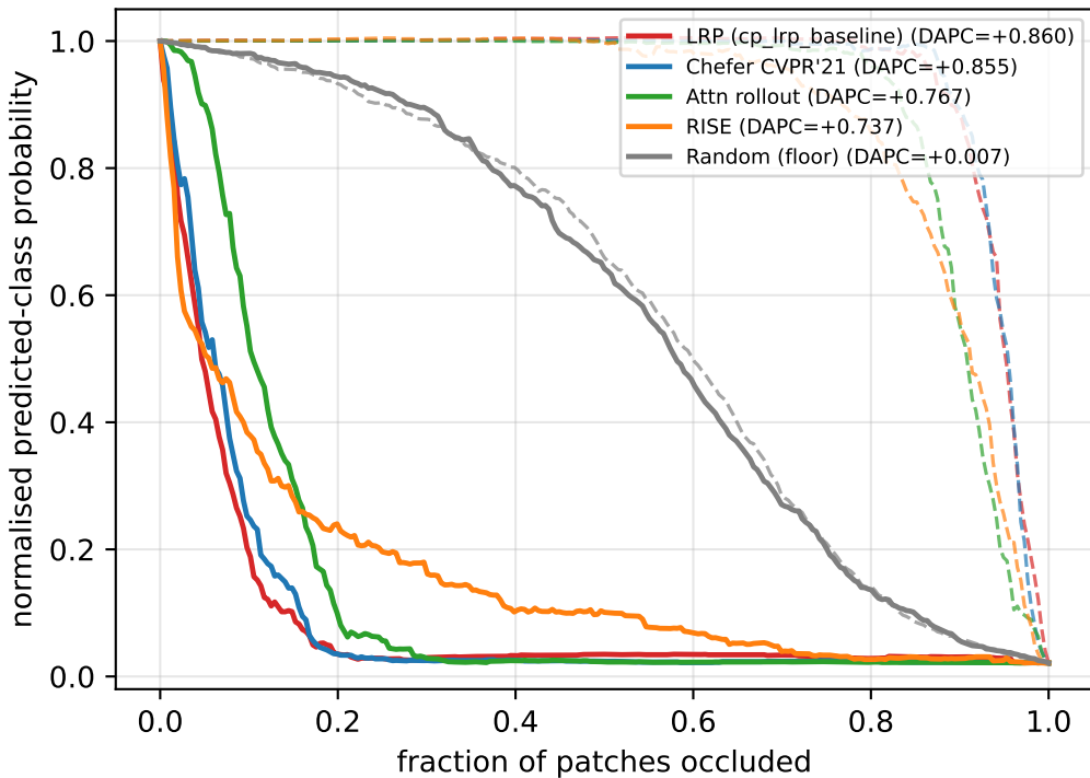
M3: DINOv3-S/16 (+reg, finetuned) · FunnyBirds (test) MoRF (solid) vs LeRF (dashed)
