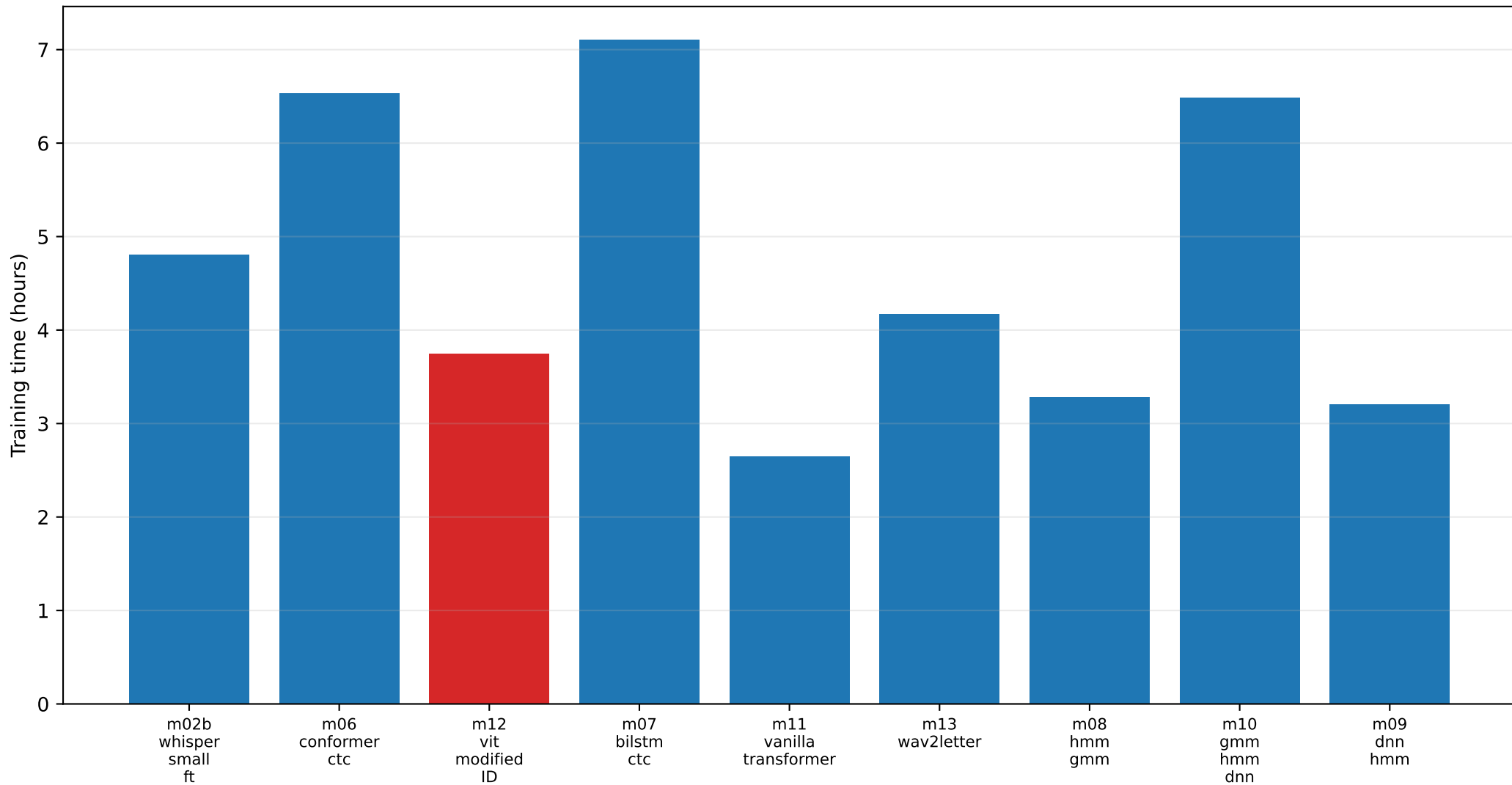
Recorded training duration by selected paper run
