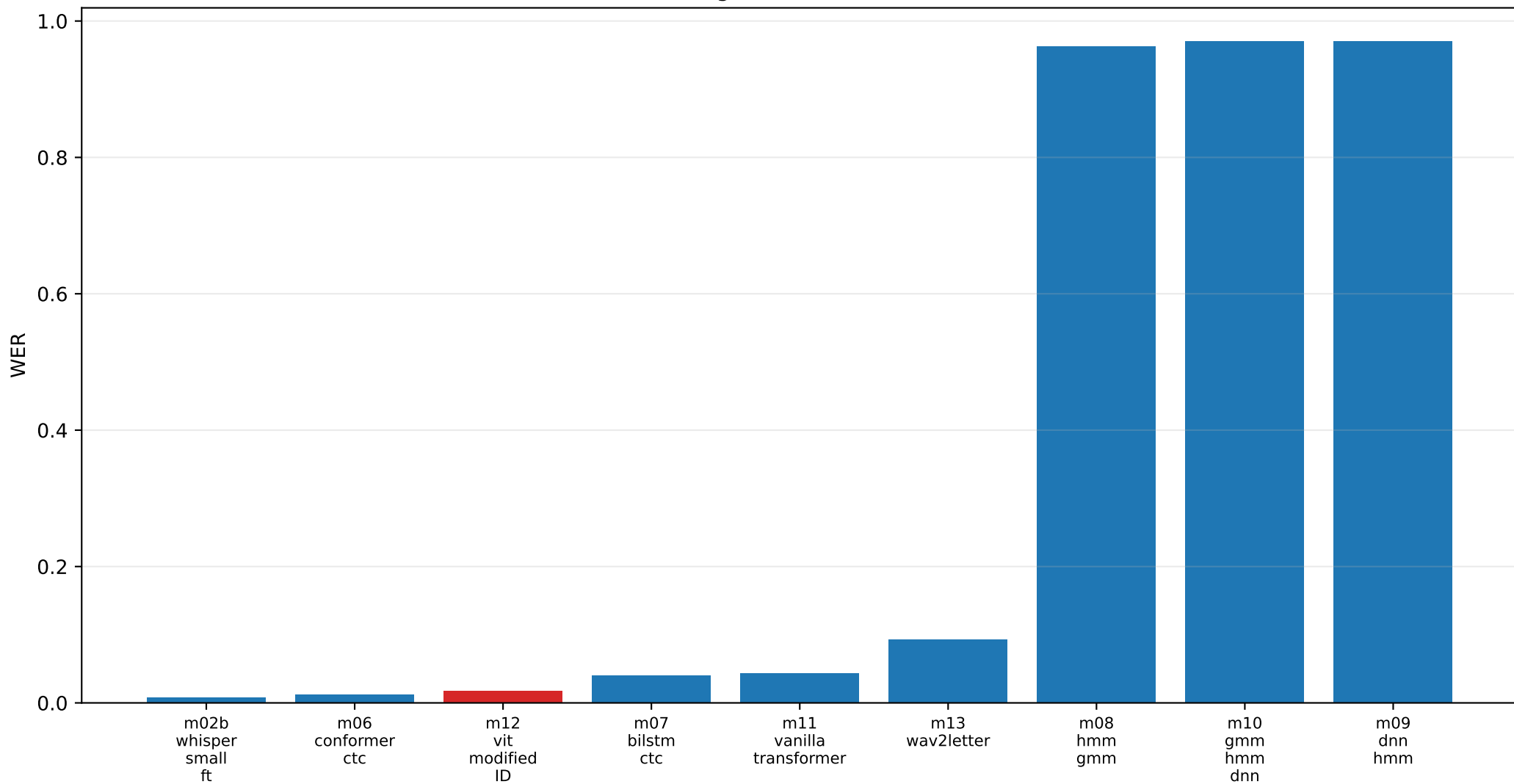
WER ranking across nine ASR models
