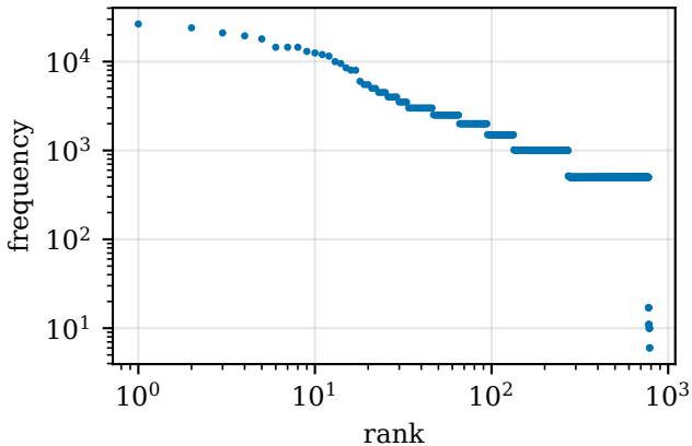
F5 Zipf rank-frequency
