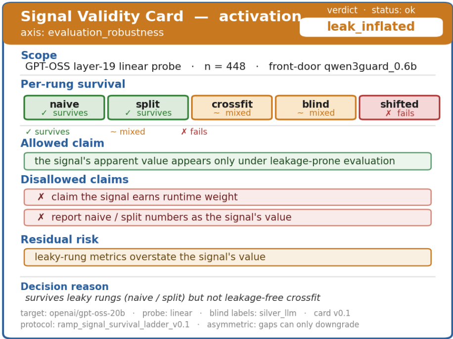
Signal Validity Card for the activation probe
