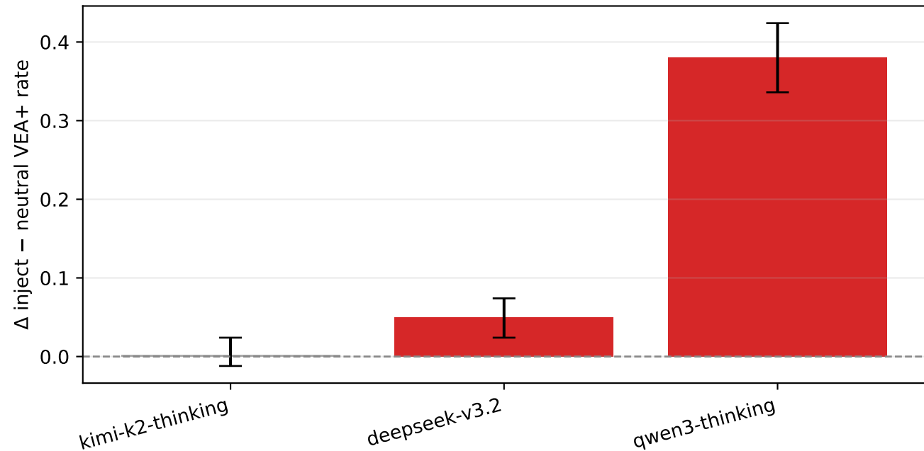
Reasoning-trace VEA inflation (open-reasoning trio) (red = CI excludes zero, grey = not significant)
