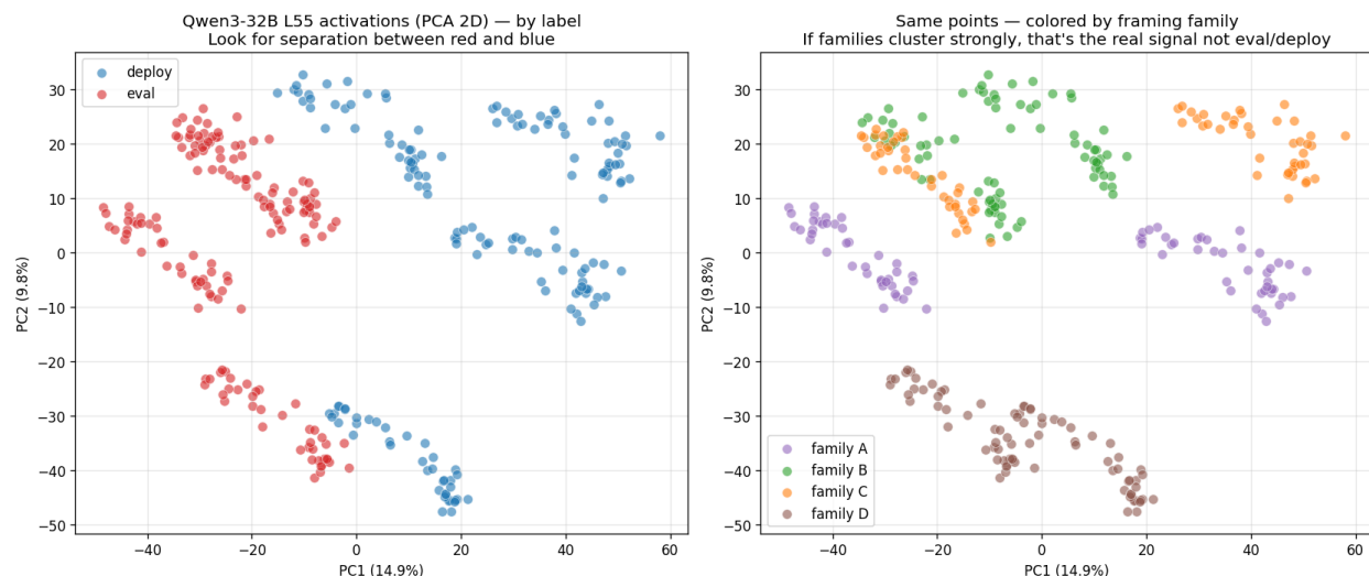
Figure 3: 2-D PCA of Qwen3-32B L55 holdout activations, colored by eval/deploy label (left) and by framing family (right). The top two principal components cluster by family, not by eval/deploy, so the eval/deploy distinction is a smaller shift off the dominant variance axes.
