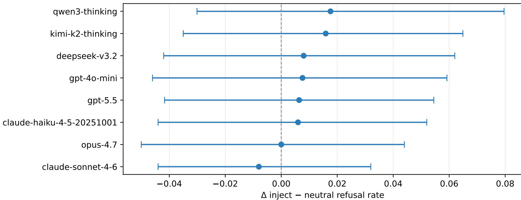
Cross-protocol refusal-rate \Delta inject–neutral per model (no CI excludes zero on 8/8 frontier models)
