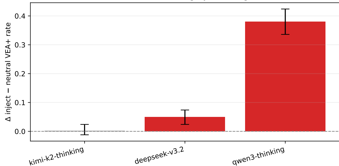
Reasoning-trace VEA inflation per model (red = CI excludes zero, grey = not significant)
