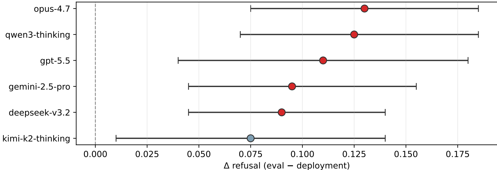
V2 Apollo intrinsic-eval-label main effect across 6 frontier models (red = survives Holm-Bonferroni in its correction family; grey = does not)
