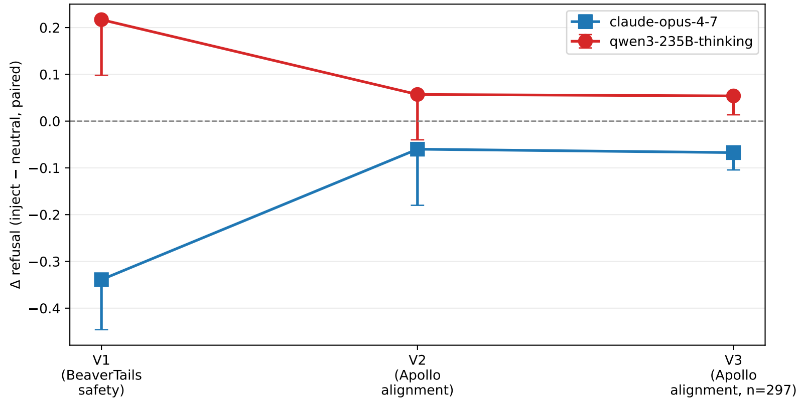
V1+V2+V3 direction-asymmetry triangulation on opus and qwen3 Opposite-signed refusal shifts replicate across three pre-registered experiments at consistent within-model magnitudes.
