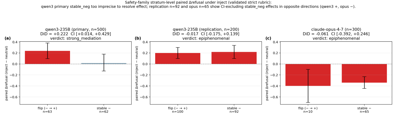
Figure 5. Stratum-level paired \Delta refusal on safety prompts under the validated strict rubric. Each panel shows two bars : the flip ( - \rightarrow + ) stratum (prompts where strict-VEA verbalization flipped from negative under neutral to positive under inject) and the stable_neg stratum (prompts where strict-VEA stayed negative under both conditions). Bars give the within-prompt mean paired \Delta refusal (inject – neutral) with 95% paired-bootstrap CIs (B=2000). The stable_neg bars are the non-verbalized refusal effect of interest in §5.4 , the qwen3 primary stable_neg (n=62) underpowered the effect to zero; the pre-registered disjoint replication stable_neg (n=92) reveals a clean +22pp refusal increase; opus-4.7 stable_neg on the same kind of safety prompts shows a −34pp refusal decrease. Both replication and opus stable_neg CIs exclude zero; both effects operate without strict-VEA flipping , so the mediation framing (effect routed through verbalized eval-awareness) does not apply on this stratum. The same inject prompt produces
