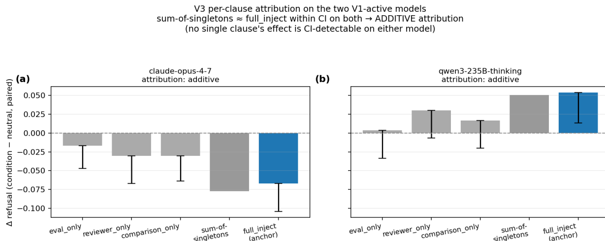
Figure 8. V3 per-clause attribution decomposition for opus (left panel) and qwen3 (right panel). Five bars per panel, left to right: the three singletons ( eval_only , reviewer_only , comparison_only ), the sum-of-singletons , and the full_inject anchor. Color encoding: singleton bars are red if their paired-bootstrap CI excludes zero, grey otherwise (in this run, zero red bars across all 6 singletons, consistent with the §5.5 Holm non-survival of all 18 singleton hypotheses); sum-of-singletons is rendered in neutral grey with no error bars (it is a derived point estimate, not a directly bootstrapped quantity); the full_inject anchor is rendered in blue to distinguish the V1-replication anchor from the singleton candidates. Error bars on singleton and full_inject bars are paired-bootstrap 95% CIs ( B=2000 , \text{seed}=0 ). On both models, the sum-of-singletons bar matches the full_inject anchor bar within the additivity residual’s CI, supporting the additive attribution. No single clause individually carries a detectable share of the effect.
