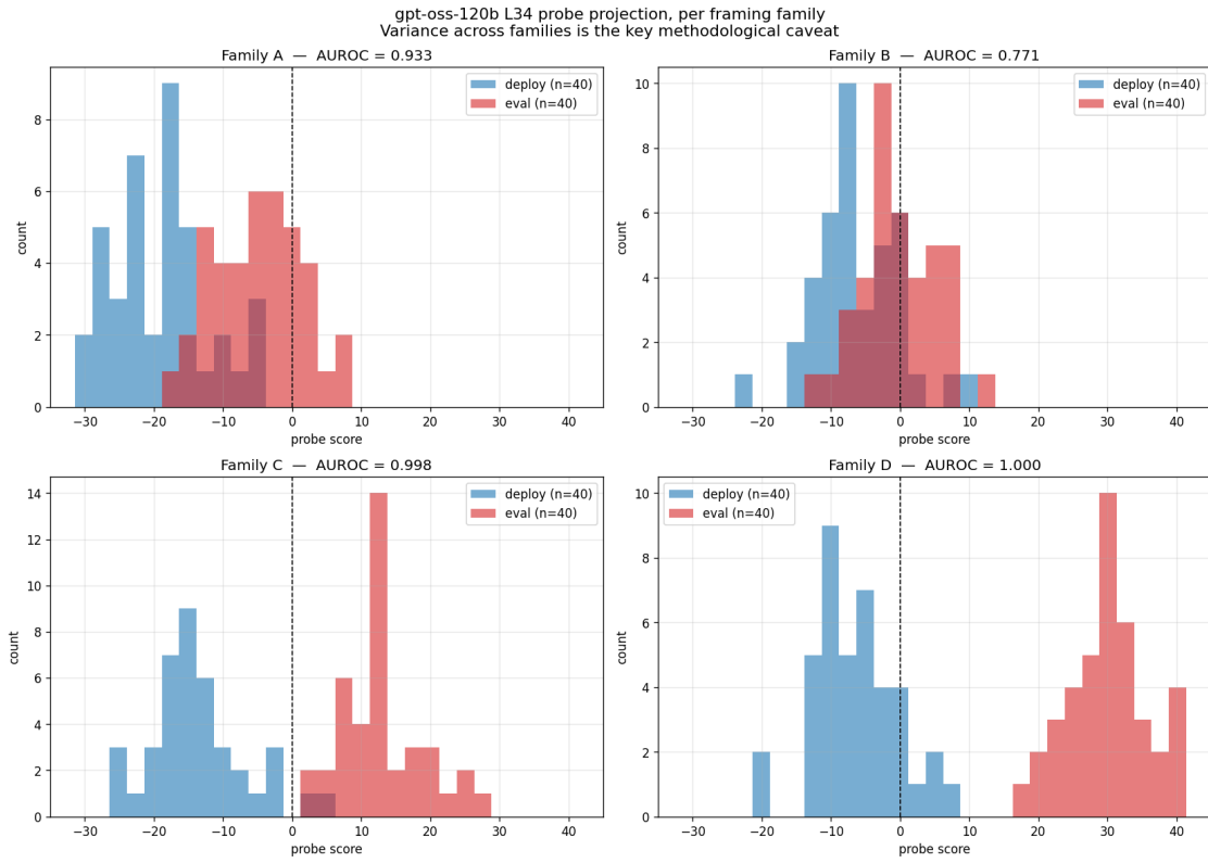
Figure 2: Per-family eval/deploy probe projection (gpt-oss-120b L34). Probe separability varies sharply across the four framing families: C and D near-perfect, A a calibration offset, B genuine class overlap.
