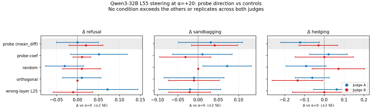
Figure 4: Steering effects at \alpha=+20 on Qwen3-32B L55: the probe direction (mean_diff, shaded) versus probe-coefficient, random, orthogonal, and wrong-layer (L25) controls, for refusal, sandbagging, and hedging (points \pm 2 SE, both judges). No condition - including the probe - is displaced from zero more than the controls, or in a way that replicates across both judges.
