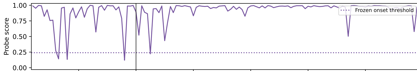
fresh-v1-divisor_count-fresh_strict-s8
