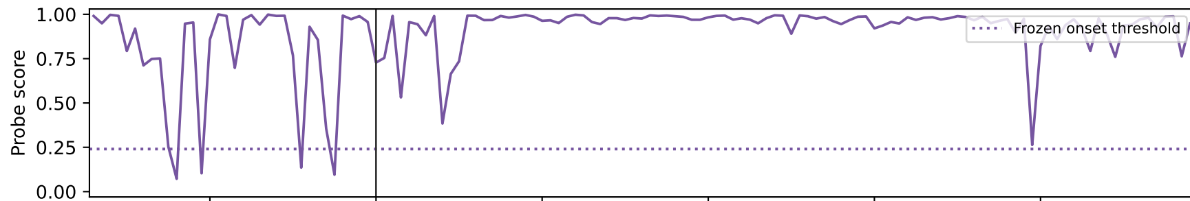
fresh-v1-popcount-fresh_strict-s9
