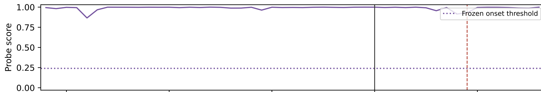
fresh-v1-rotate_array-source_dont_hack-s5
