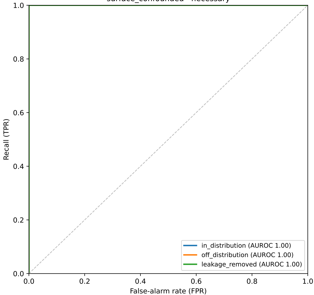
SIEVE deployment ROC surface_confounded · necessary
