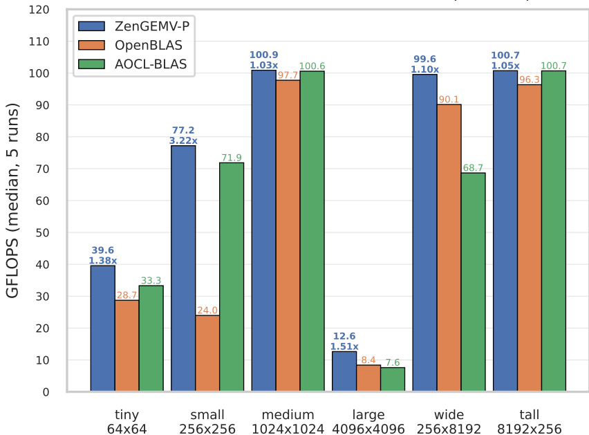
Multi-Threaded GEMV Performance (6 cores)
