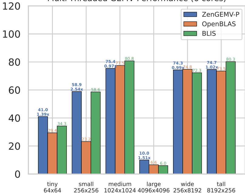
Multi-Threaded GEMV Performance (6 cores)
