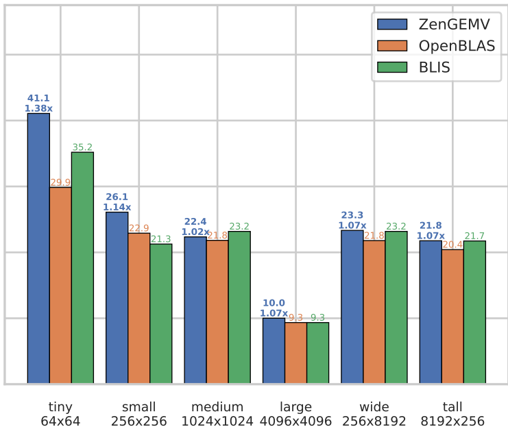
Single-Threaded GEMV Performance
