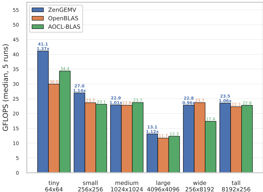
Single-Threaded GEMV Performance
