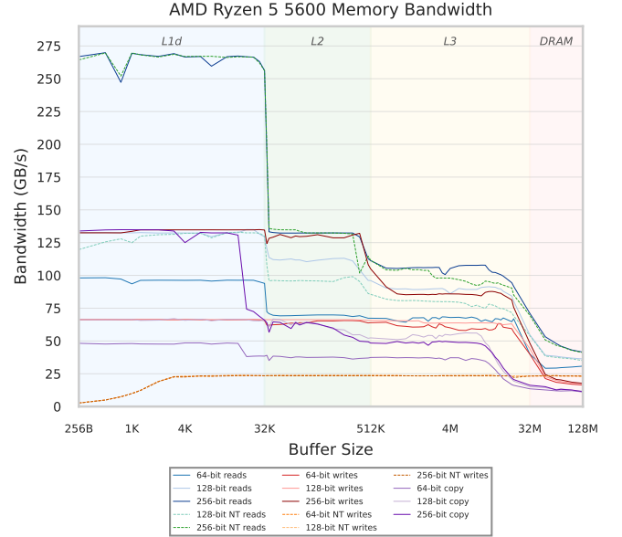
Fig. 1. Memory bandwidth measured with the bandwidth tool [15] on the AMD Ryzen 5 5600 for sequential reads, writes, nontemporal (NT) operations, and copies at 64/128/256-bit widths. The shaded regions mark cache levels: L1d ( \sim 267 \text{ GB/s} peak read), L2 ( \sim 132 \text{ GB/s} ), L3 ( \sim 106 \text{ GB/s} ), and DRAM ( \sim 42 \text{ GB/s} ).
