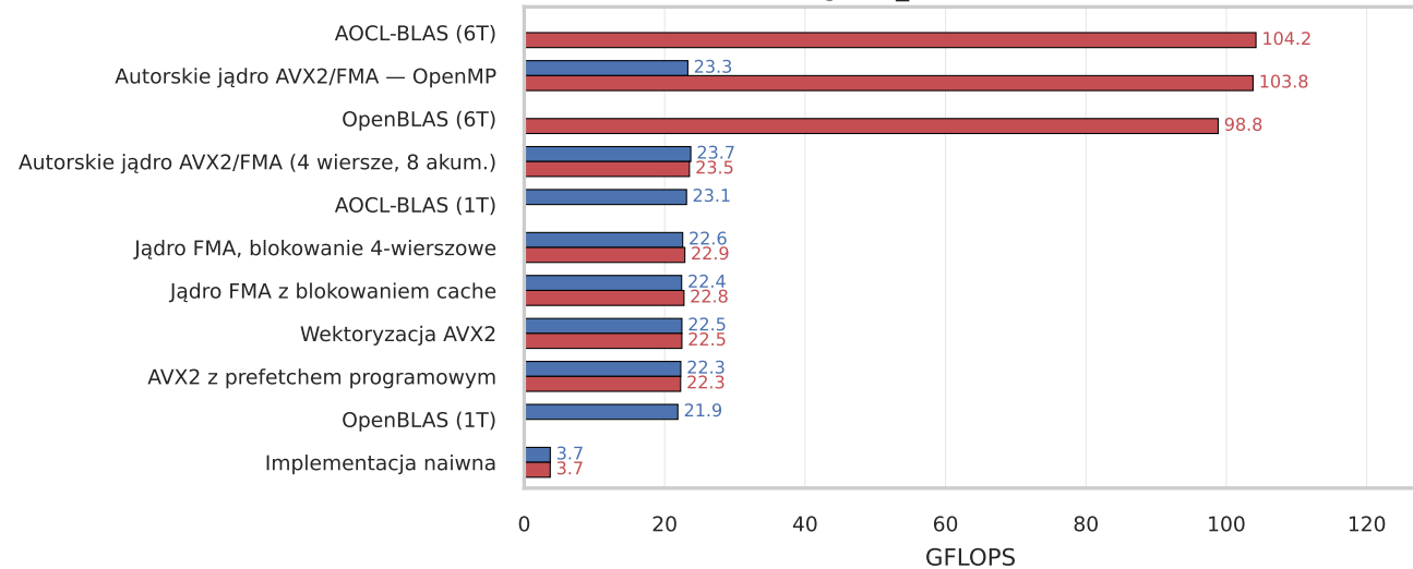
gemv_tall (8192x256)
