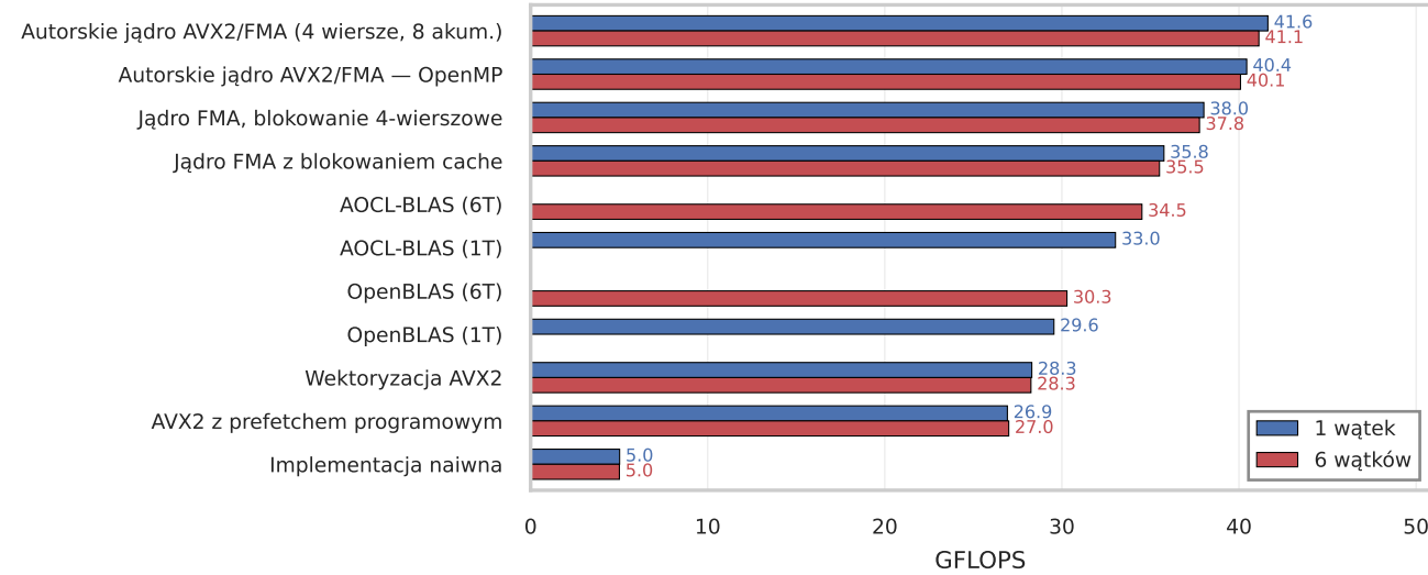
gemv_tiny (64x64)
