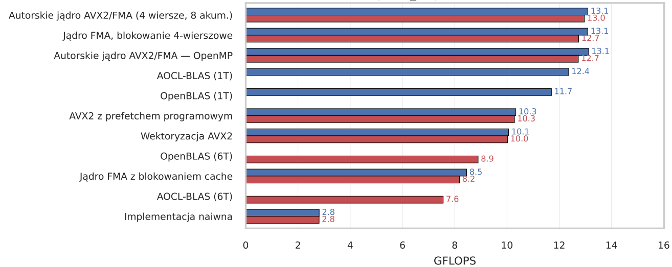
gemv_large (4096x4096)
