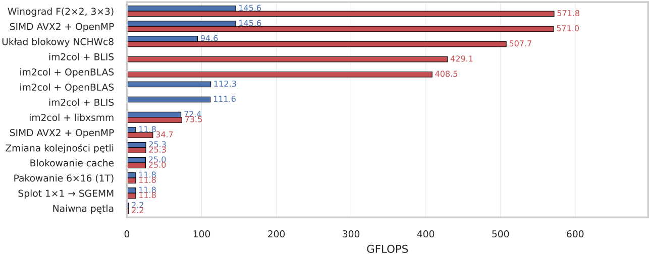
conv_small (Cin=64 HxW=56x56 K=3 Cout=64)
