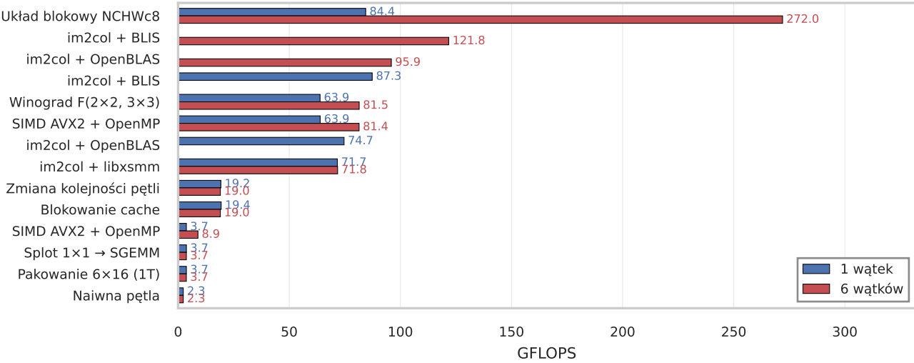
conv_tiny (Cin=16 HxW=32x32 K=3 Cout=16)
