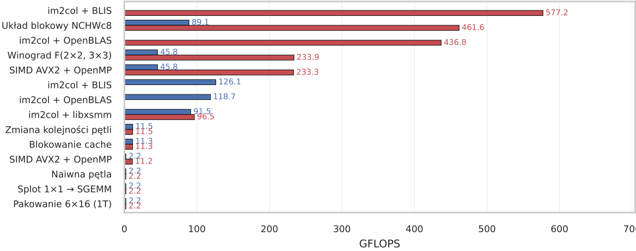
conv_large (Cin=256 HxW=14x14 K=3 Cout=256)
