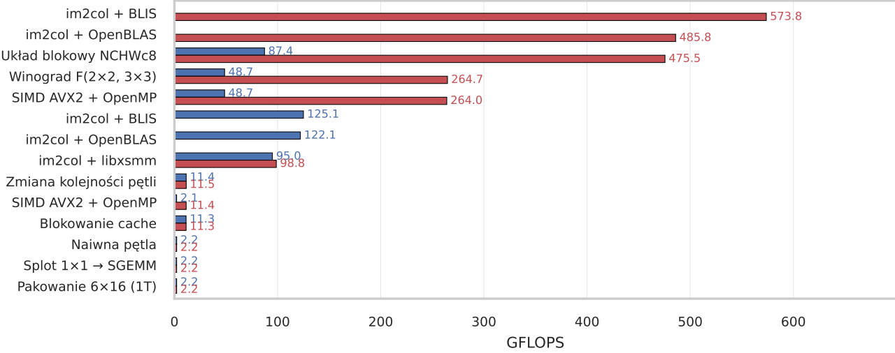
conv_xlarge (Cin=512 HxW=14x14 K=3 Cout=512)
