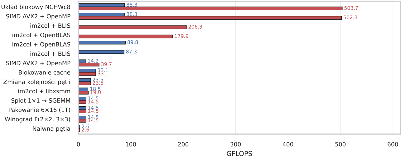
conv_kernel7 (Cin=64 HxW=112x112 K=7 Cout=64)
