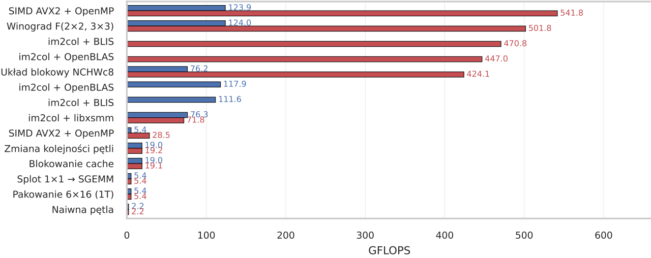
conv_mid (Cin=128 HxW=28x28 K=3 Cout=128)
