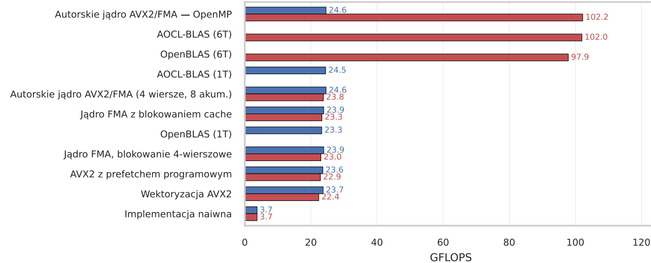
gemv_tall (8192x256)
