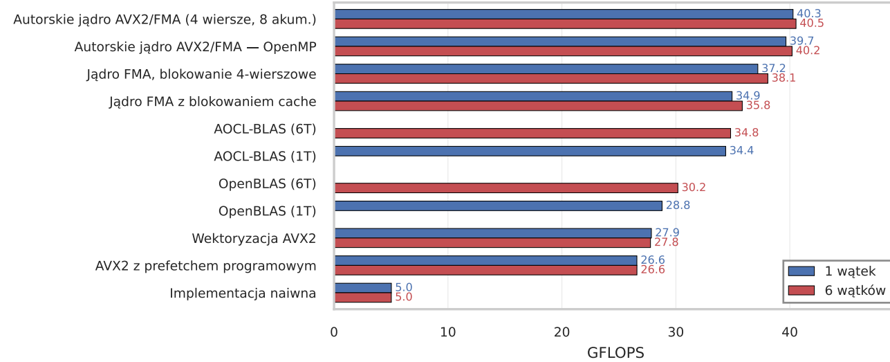
gemv_tiny (64x64)
