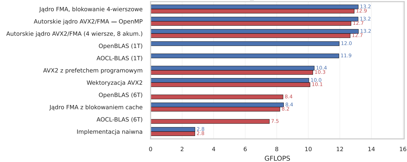
gemv_large (4096x4096)
