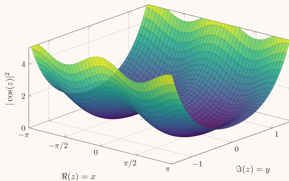
Magnitude Squared of the Complex Cosine Function
