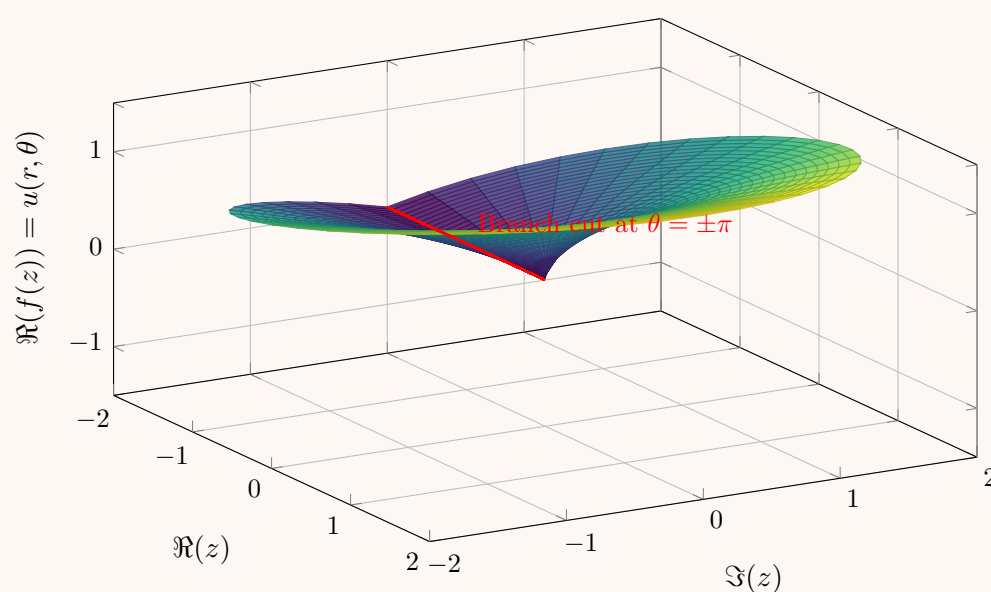
Branch Cut Visualization of f(z) = \sqrt{z}
