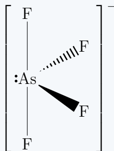
See-Saw Shape ( sp^3d )
