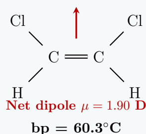
cis -1,2-dichloroethene
