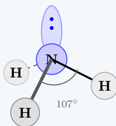
Trigonal Pyramidal ( sp^3 )
