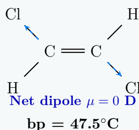
trans -1,2-dichloroethene
