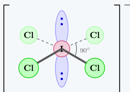
Square Planar ( sp^3d^2 )
