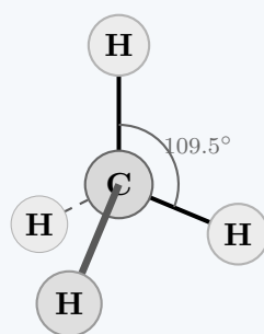
Tetrahedral ( sp^3 )
