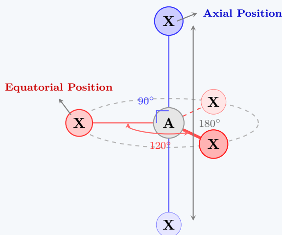
Trigonal Bipyramidal Geometry ( sp^3d )
