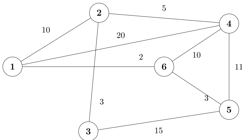
Figure 1: Weighted Graph
