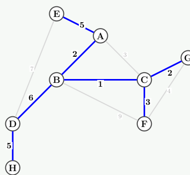
Step 6: Add BD(6) (Final MST)
