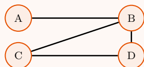
Graph G (IS = {A, C})
