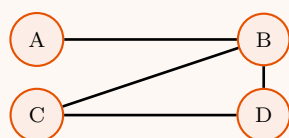
Graph G (IS = {A, C})
