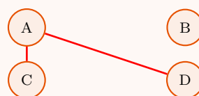
Graph \bar{G} (Clique = {A, C})
