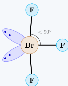
T-shaped ( sp^3d )
