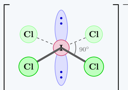
Square Planar ( sp^3d^2 )
