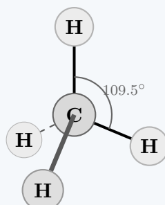
Tetrahedral ( sp^3 )
