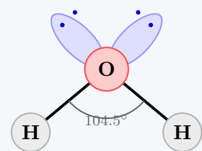
Bent / V-shaped ( sp^3 )
