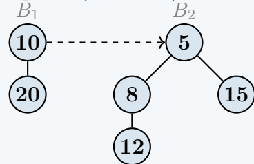
Heap H_1 (6 nodes)
