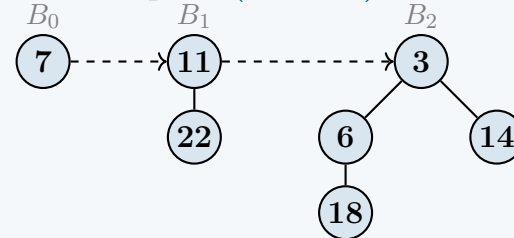
Heap H_2 (7 nodes)
