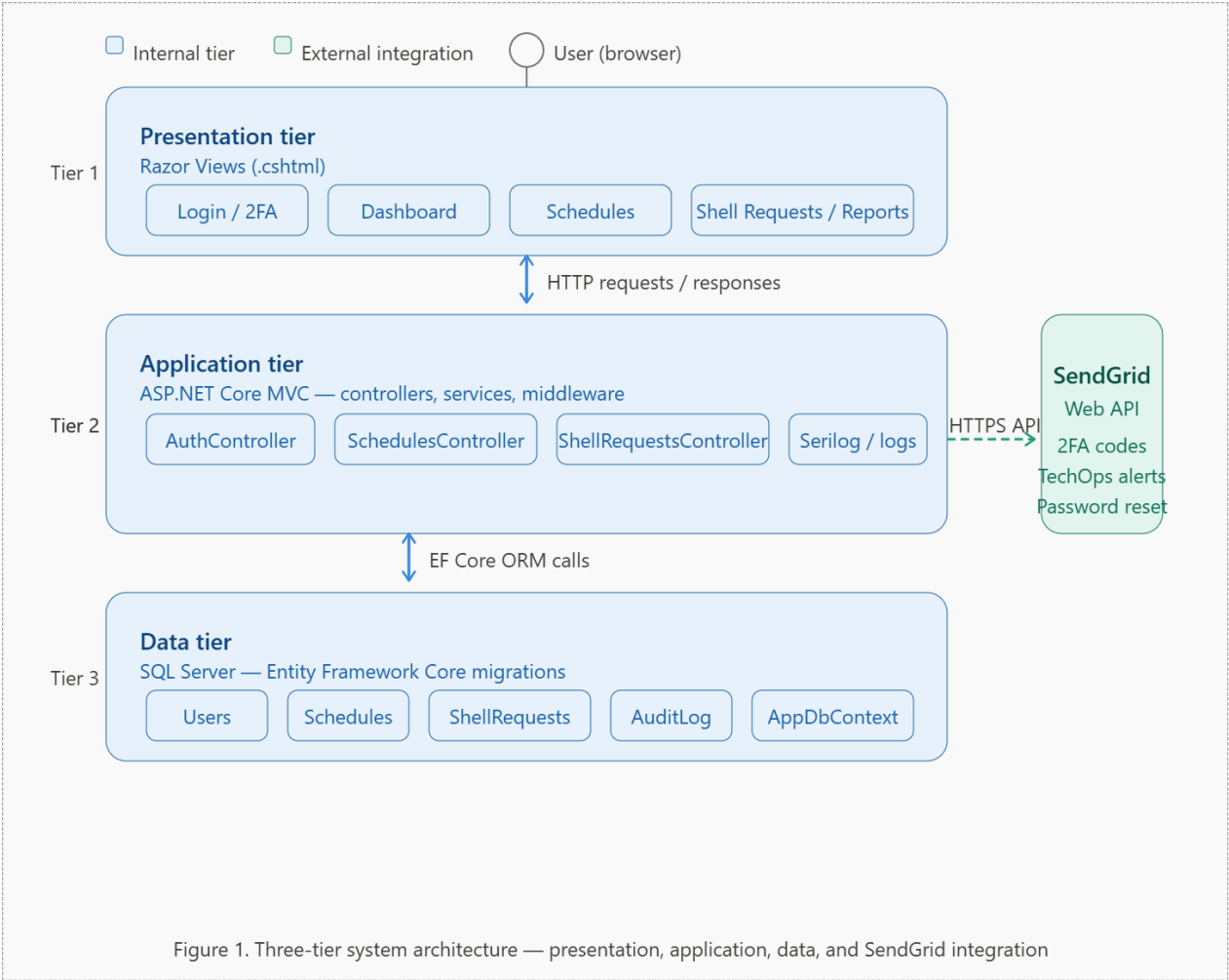
Figure 1. Three-tier system architecture showing presentation, application, data, and SendGrid integration layers
