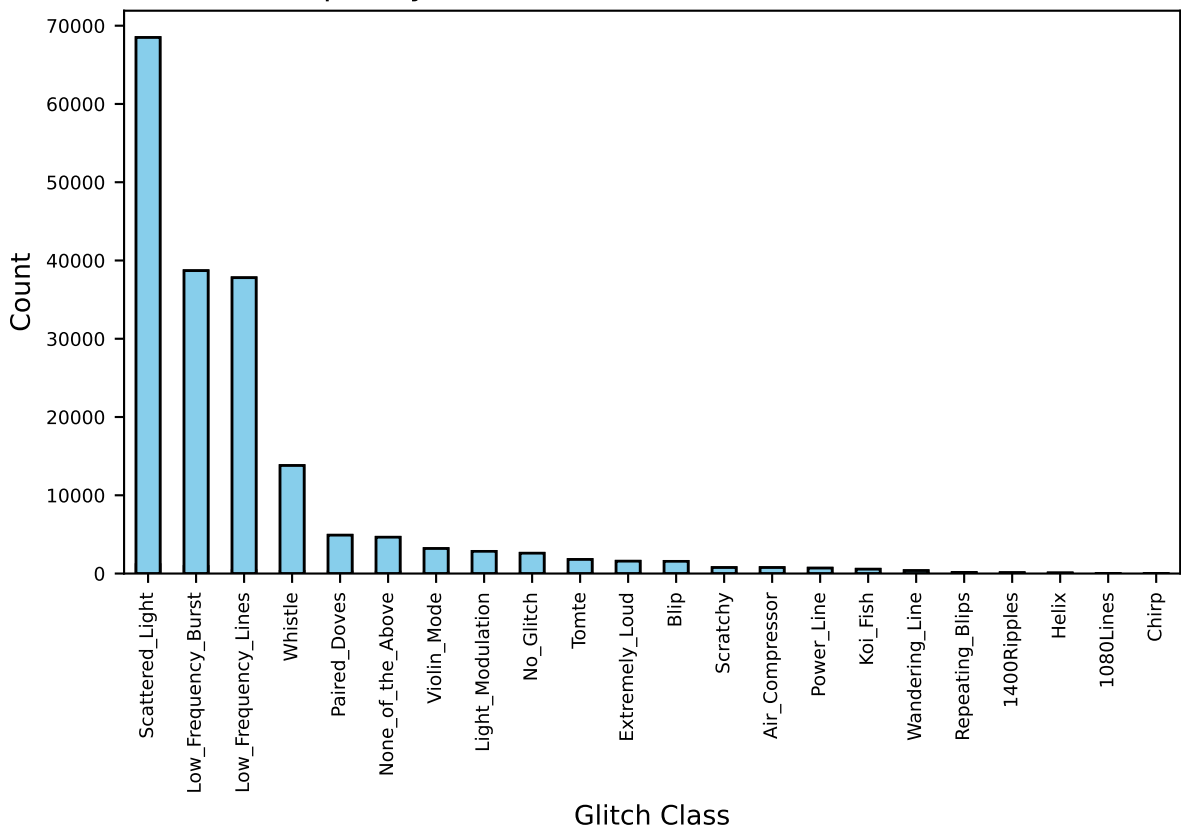
Frequency of Unmatched Glitches (seismic data)
